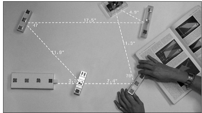
Figure 2 The tangible Illuminating Light workbench lets students learn about optical systems by designing them.
