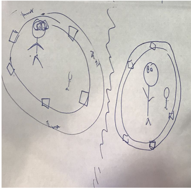
Virtual Reality
