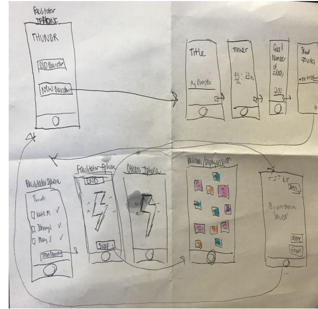
IOS Application
