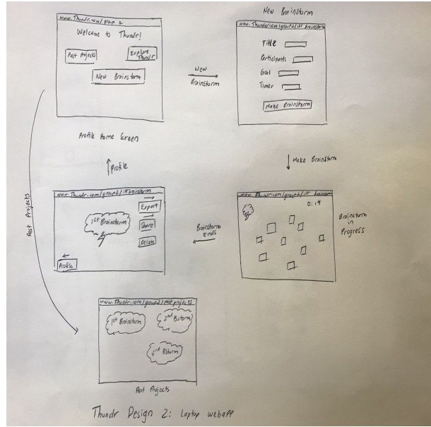
Web Application
