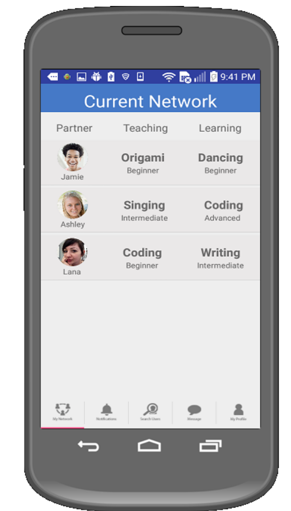
Hi-fi prototype
