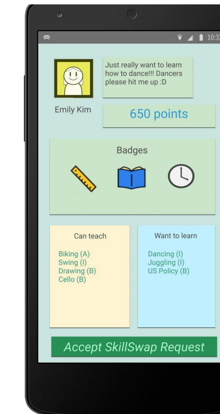
Med-fi prototype
