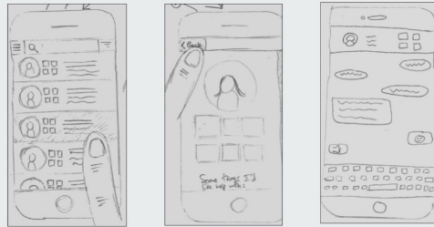
Low-Fi Prototyping
