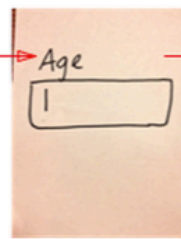
Fig. 4: Age entry
